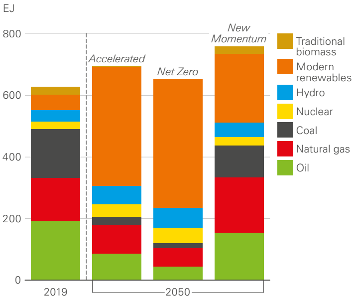
Primary energy by fuel
