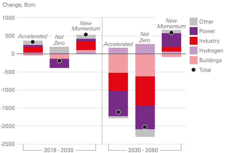
Natural gas demand by sector
